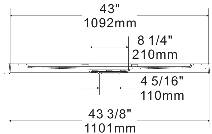
Freestanding shower base 42"x42"
